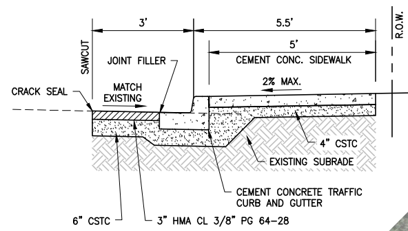
1 TYPICAL SIDEWALK SECTION N.T.S.
